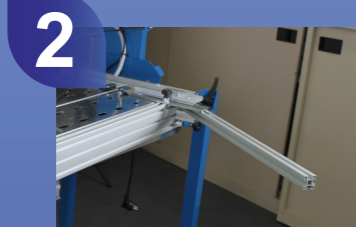
2 Foldable support arms for larger tiles
